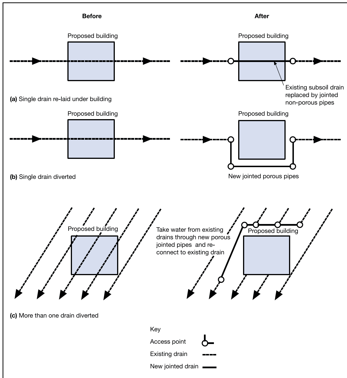
Diagram 3 Subsoil drain cut during excavation
